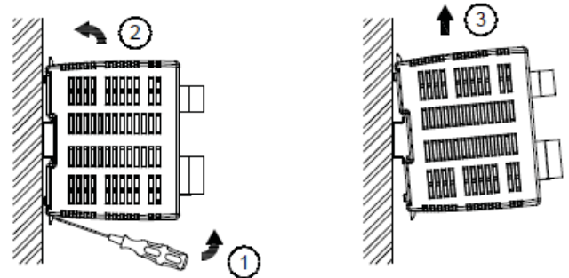
Fig. 2.2 Dismounting
