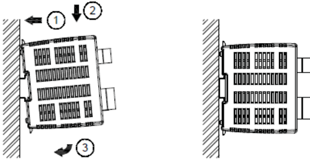
Fig. 2.1 Mounting
