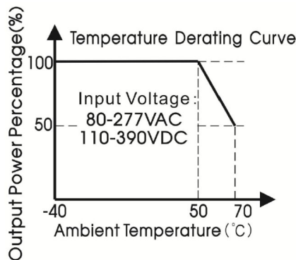
DERATING CURVE
